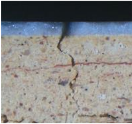
Figure 13 - Section through a crazing crack propagating into the biscuit
