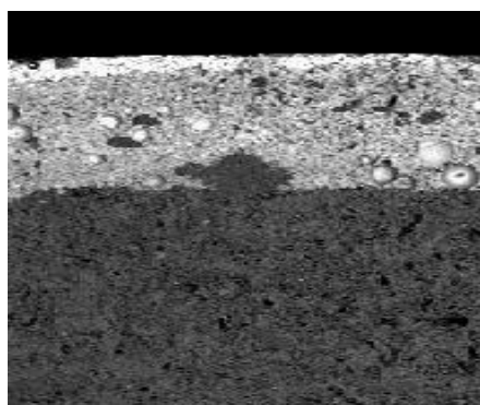
Figure 7 - SEM image of a sound azulejo glaze/biscuit interface
