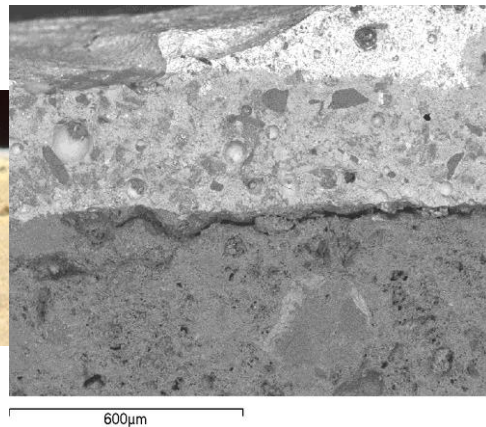
Figure 10 - SEM image of glaze detachment
