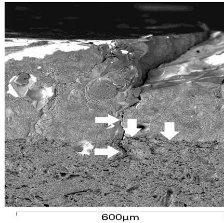
Figure 14 - SEM image of a crazing crack propagating mostly into the glaze interface
