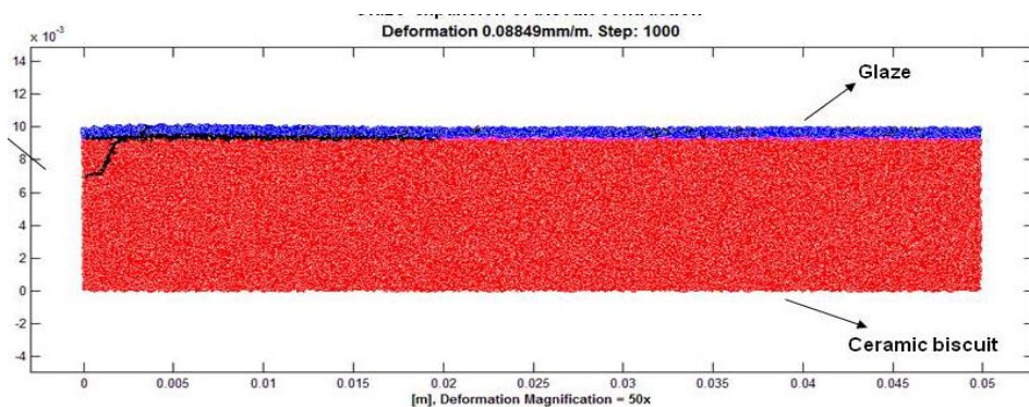
Figure 15 - One step of the graphic result of a numerical model of cooling tile shivering
