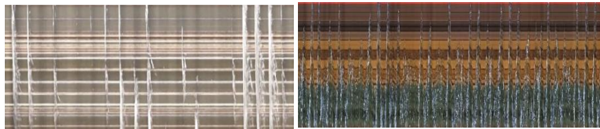
Fig. 2. TimeStack images for identifying overtopping (left) and run-up events (right).
