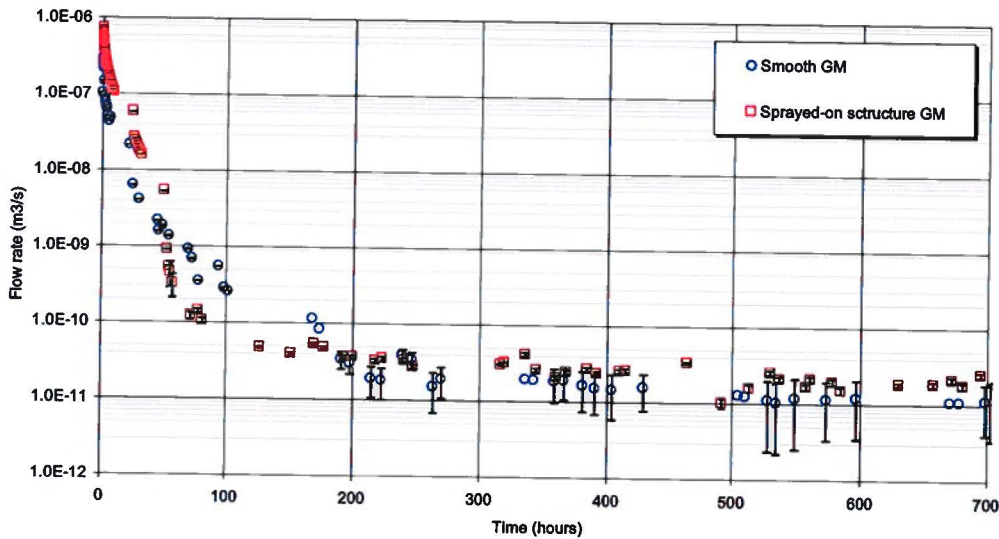
Figure 4. Comparison between the evolutions of flow rates in tests conducted with the smooth and sprayed-on structure GMs
