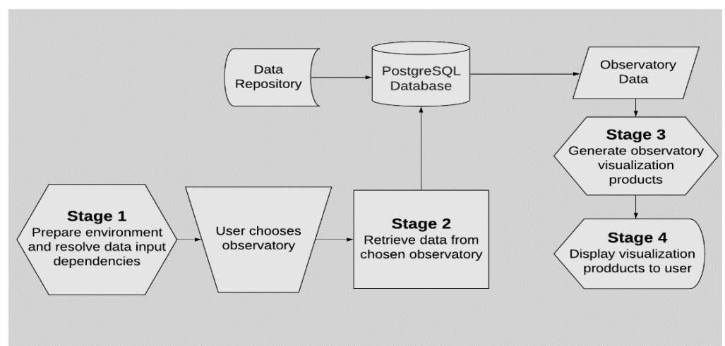
Figure 5. MOSAIC platform workflow.
