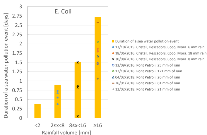
Figure 28. Duration of sea water E. Coli contamination as a function of the rainfall volume.
