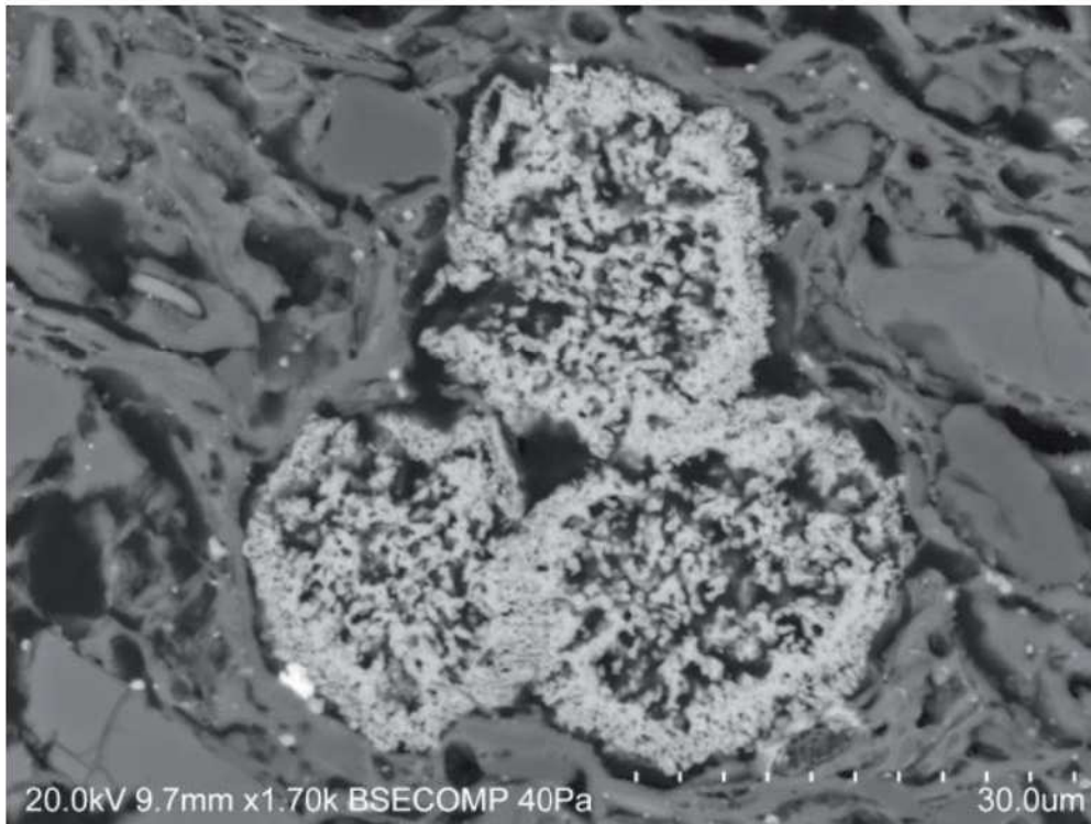
Figure 7: Annular framboids (Az 032/07)
