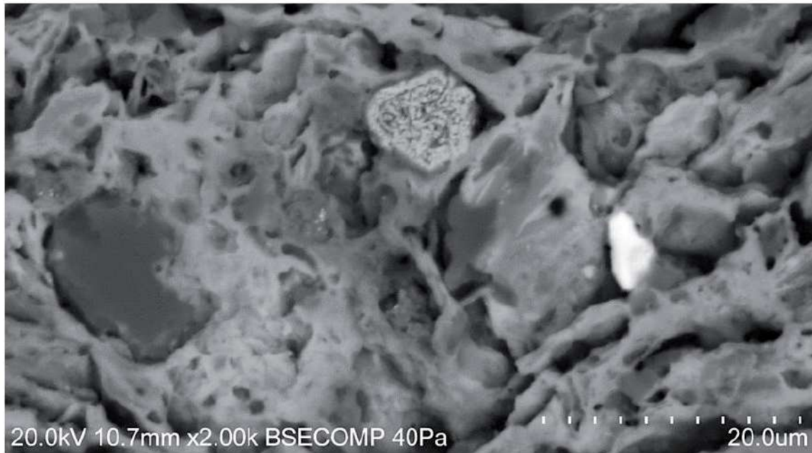
Figure 9: Euhedral-shaped crystal with framboidal core (sample Az032/04)
