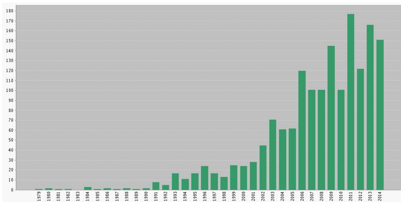
Figure 1 - Evolution of the research in estuarine and coastal morphodynamics: number of papers per year referenced in the Science Citation Index Expanded until 2014 (search string: Topic=((estuar* or coast* or inlet* or beach) and (morphodynamic or morphodynamics)) ), performed on March 10, 2015). The peaks in 2009 and 2011 are partly explained by the large number of papers published on the subject in the special issues of the Journal of Coastal Research associated with the International Coastal Symposiums that occurred in those years. These papers originate mostly from the USA, Europe (Netherlands, England, France, Spain, Italy, Portugal and Germany), Brazil and Australia
