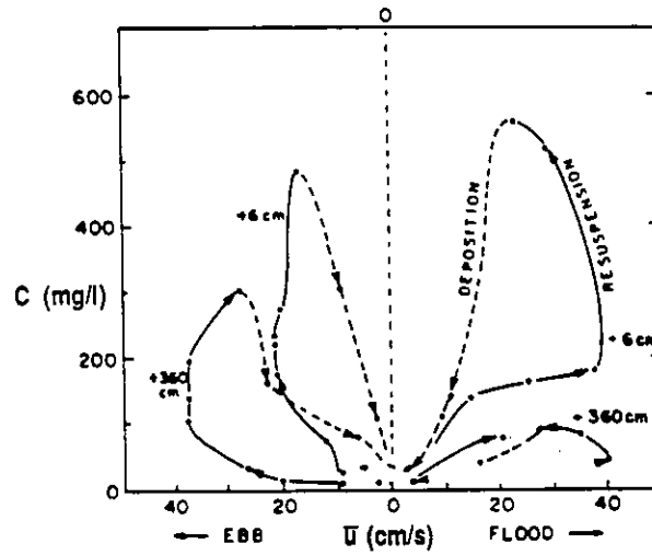
Figure 5.7: Flow-sediment hysteresis. Resuspension, solid lines; deposition/settling, dashed lines; indeterminate, dotted lines. From Nichols (1986).
