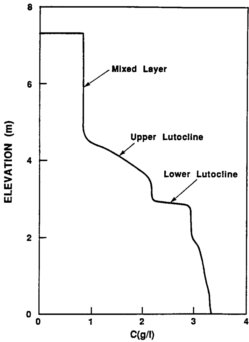
Figure 5.1: Initial concentration profile.
