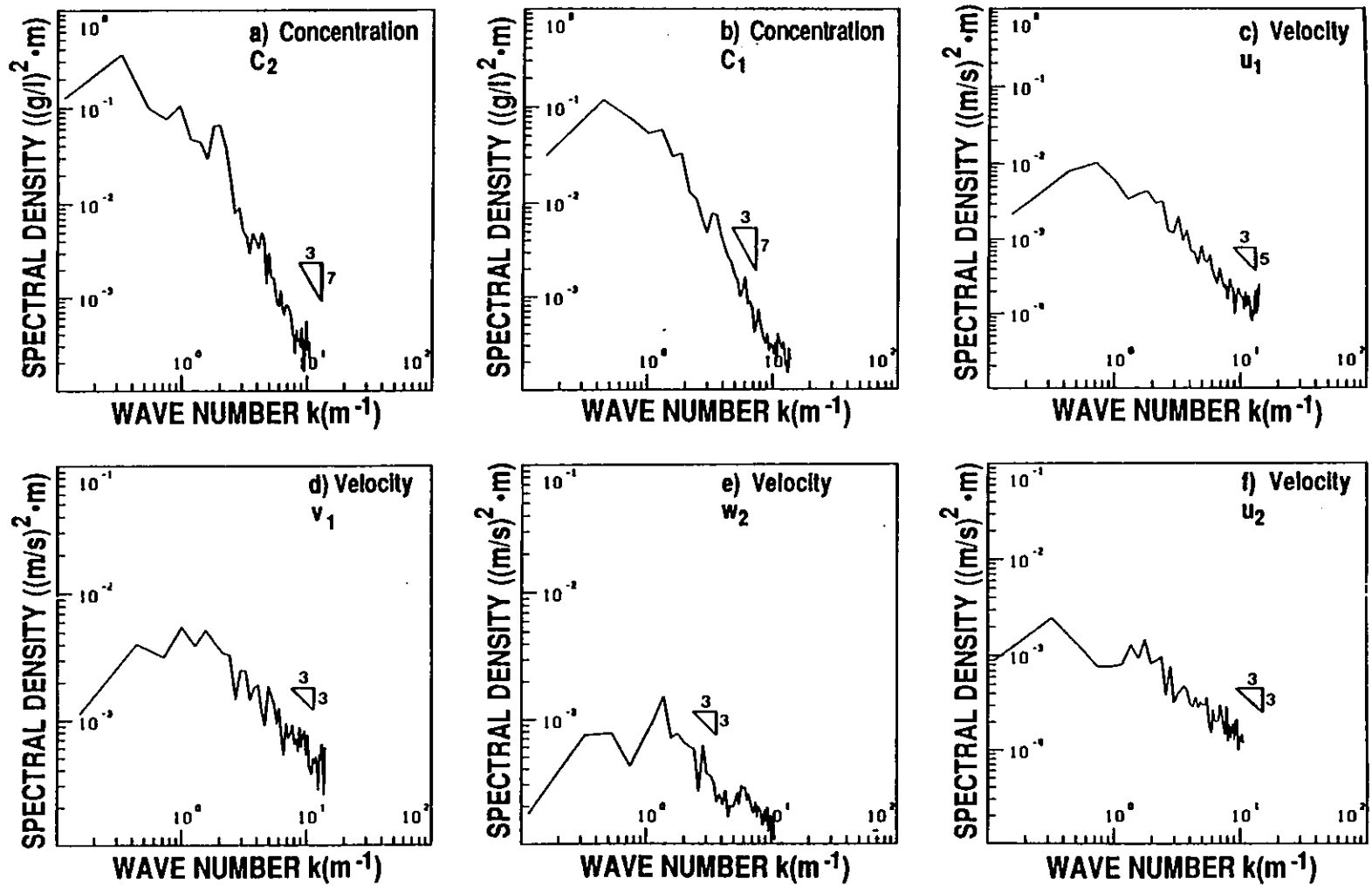
Figure 5.17: Examples of computed spectra for variables of the e' type. a) C_2 ; b) C_1 ; c) u_1 ; d) v_1 ; e) w_2 ; f) u_2
