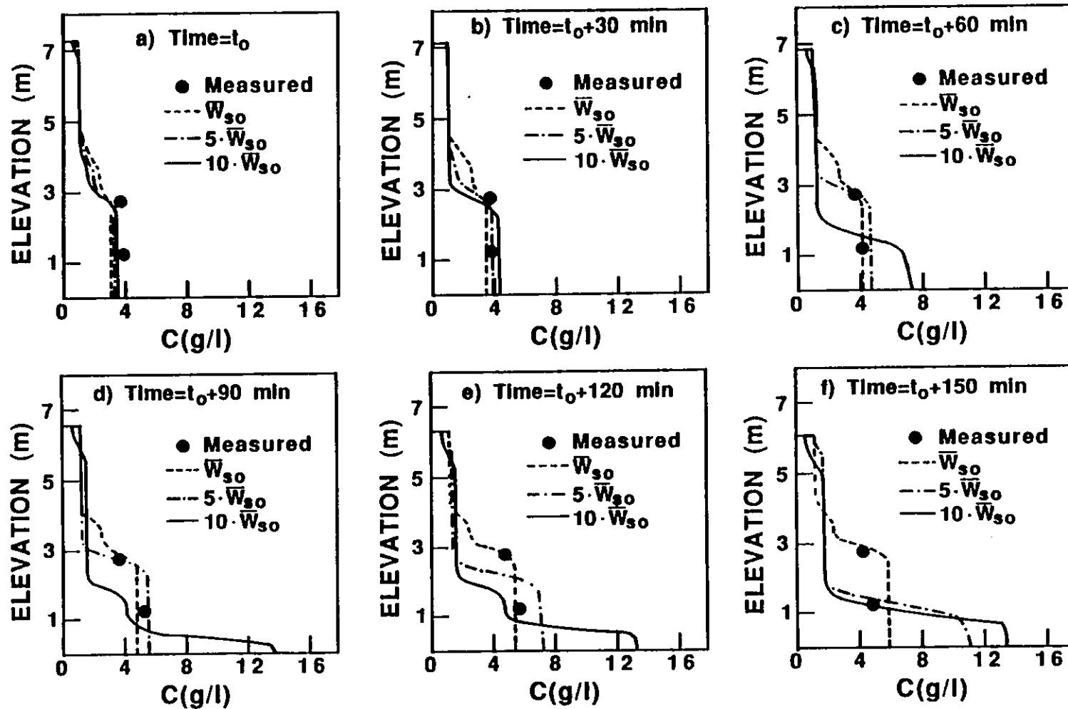
Figure 5.2: Simulated profiles with different settling velocities.
