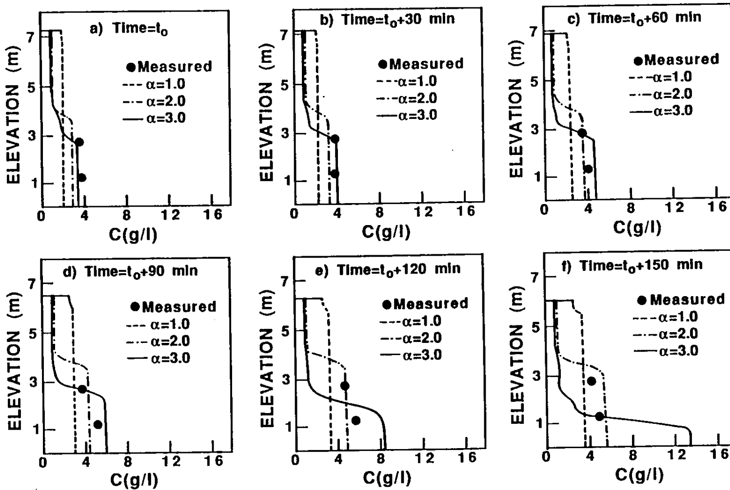
Figure 5.4: Simulated profiles with different values of diffusion parameter \alpha .
