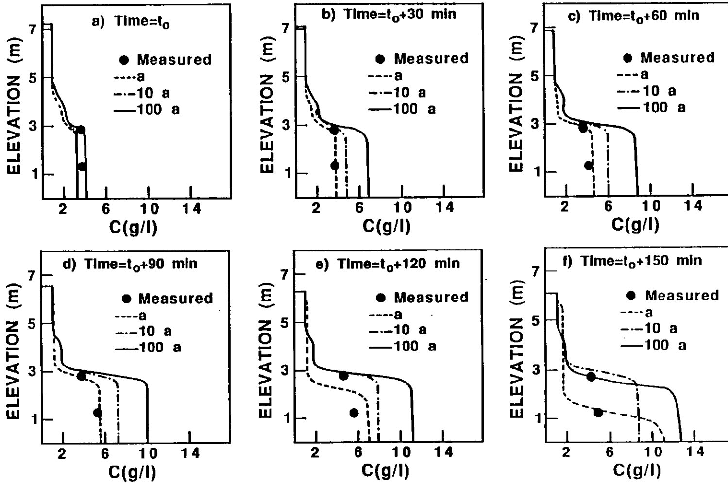
Figure 5.3: Simulated profiles with different erosion conditions.
