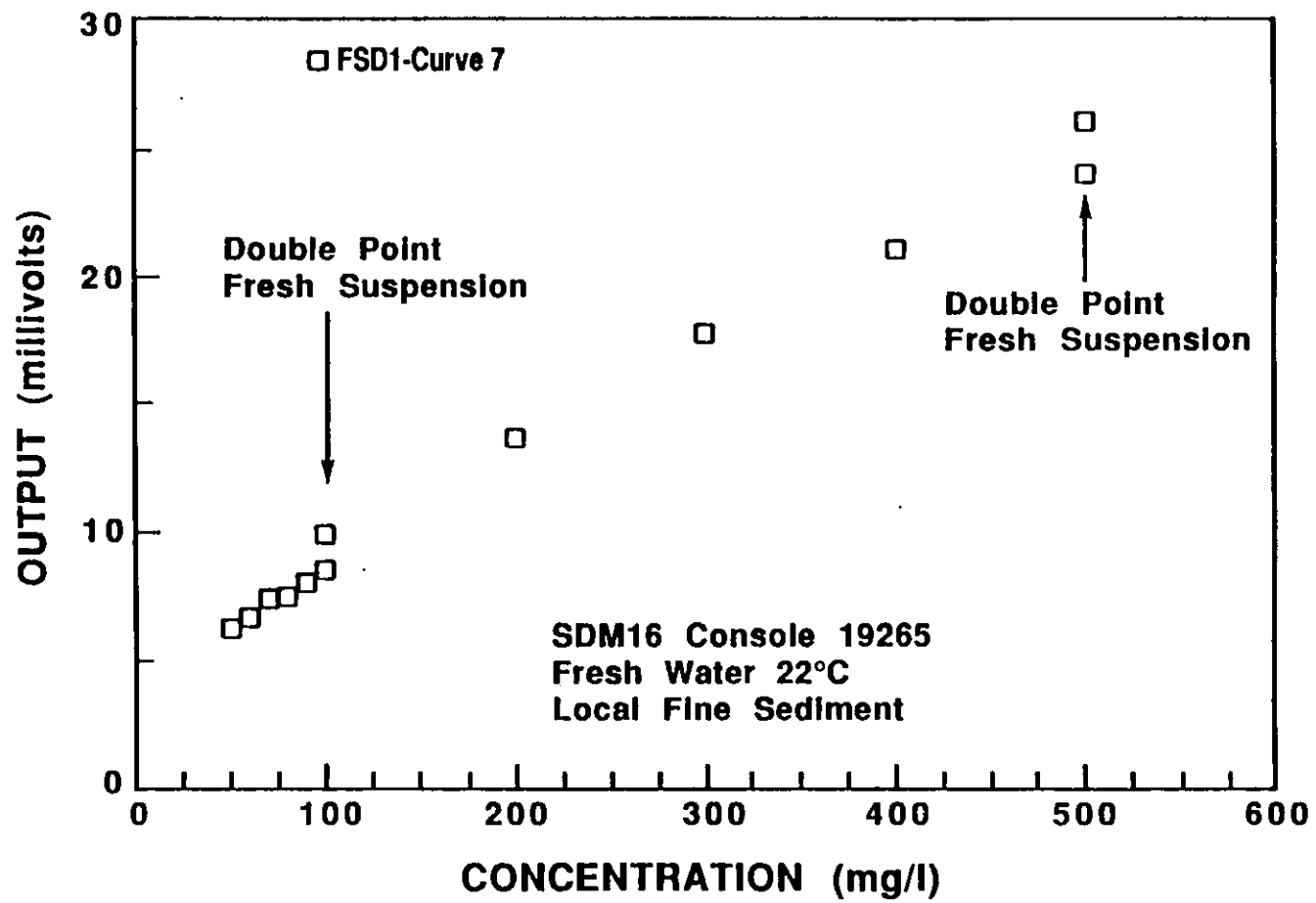
Figure A.3: Calibration curve for the SDM16 transducer and FSD1 channel of console 19265 using fresh water.
