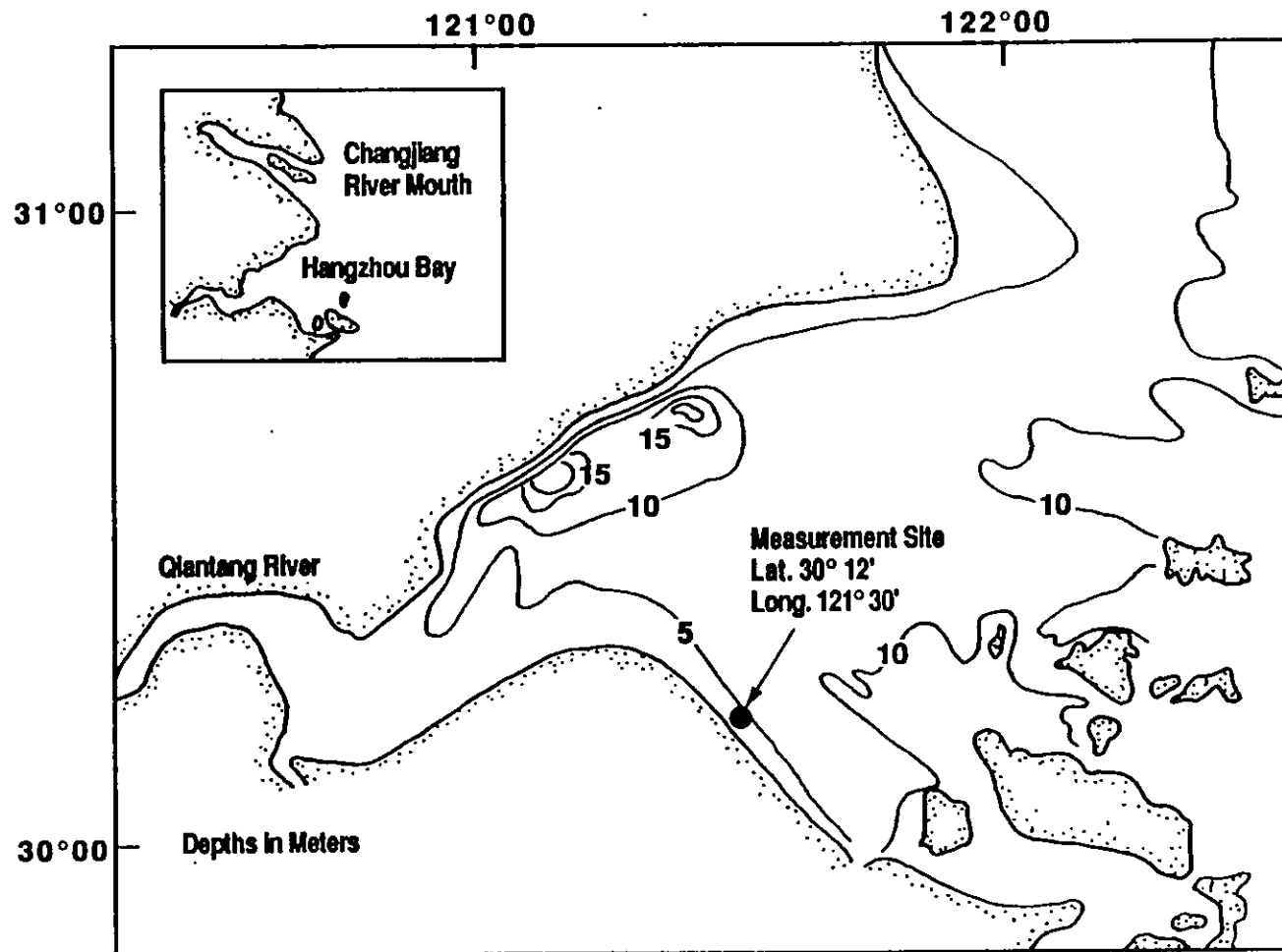
Figure 4.4: Location of the measurement site in Hangzhou Bay.
