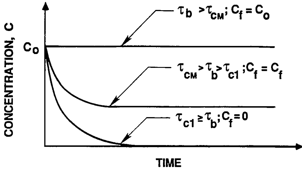
Figure 3.4: Typical time concentration relationship during deposition. From Mehta and Lott, 1987.
