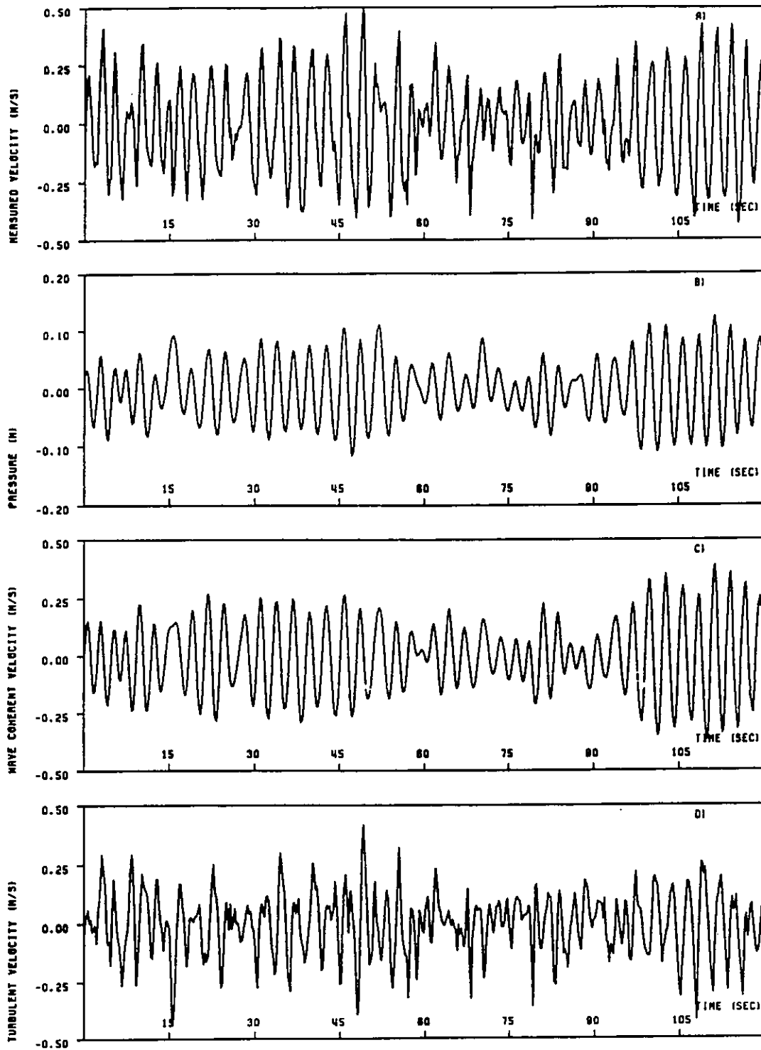
Figure 4.8: Examples of the filtering procedure applied to the measured u_2 , velocity data at the upper level (Deployment C3, block 7). a) measured u_2 ; b) pressure record; c) \tilde{u}_2 ; d) u'_2 .
