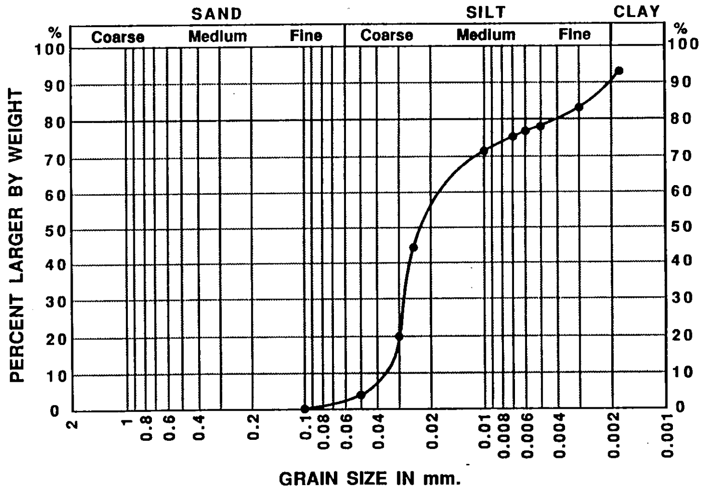
Figure 4.1: Grain size distribution.
