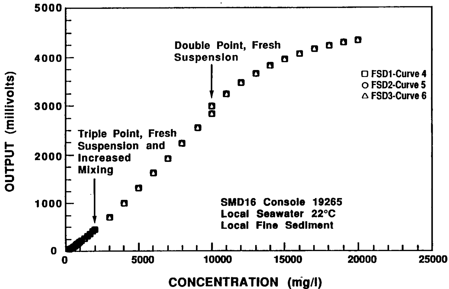
Figure A.2: Calibration curves for the SDM16 transducer and console 19265 using saline water.
