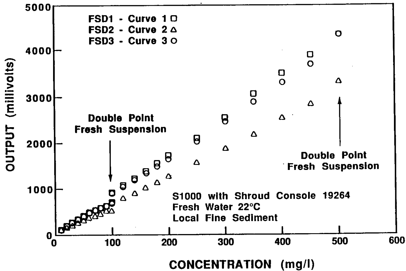
Figure A.1: Calibration curves for the S1000 transducer and console 19264 using fresh water.
