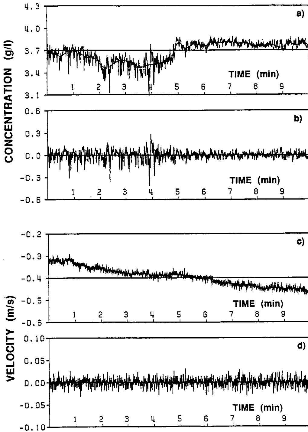
Figure 4.7: Trend removal from the measured records (deployment C2, data block 2). a) Measured c_2 (upper level); b) c_2 after trend removal; c) measured u_2 (upper level); d) u_2 after trend removal.
