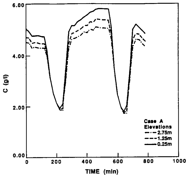
Figure 5.11: C vs. time for case A.
