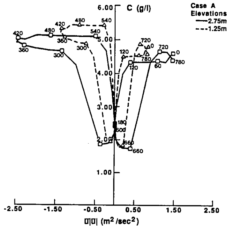
Figure 5.10: C vs. \bar{u}|\bar{u}| for case A.
