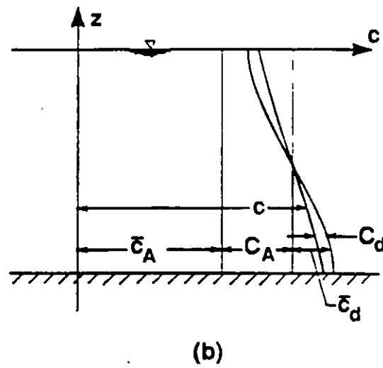
Figure 2.2: Decomposition of two-dimensional profiles into components: a) velocity; b) concentration. Adapted from Fischer, 1972.
