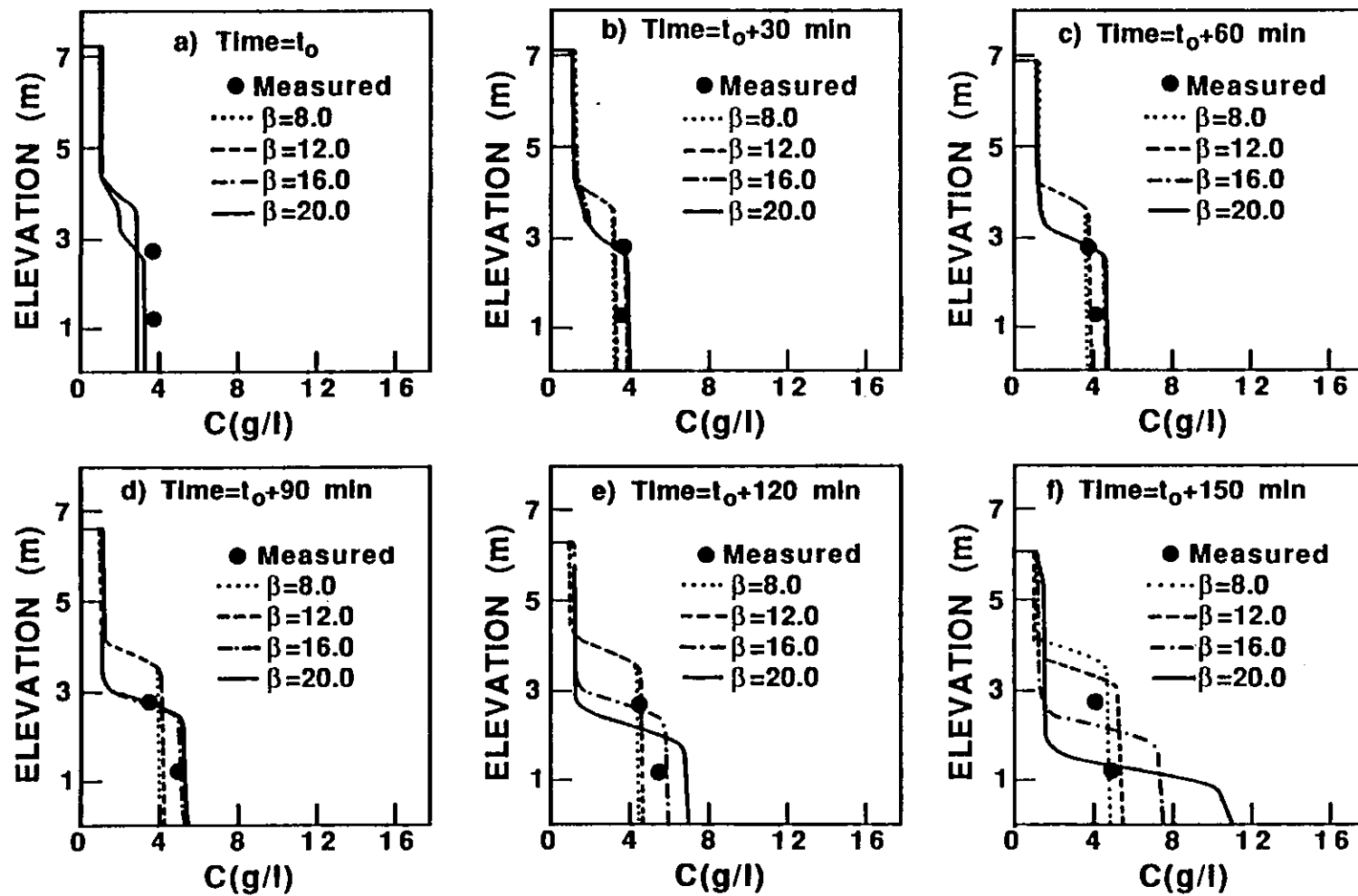
Figure 5.5: Simulated profiles with different values of diffusion parameter \beta .
