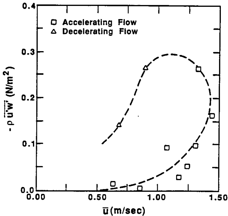
Figure 5.20: Hysteresis in Reynolds stresses.
