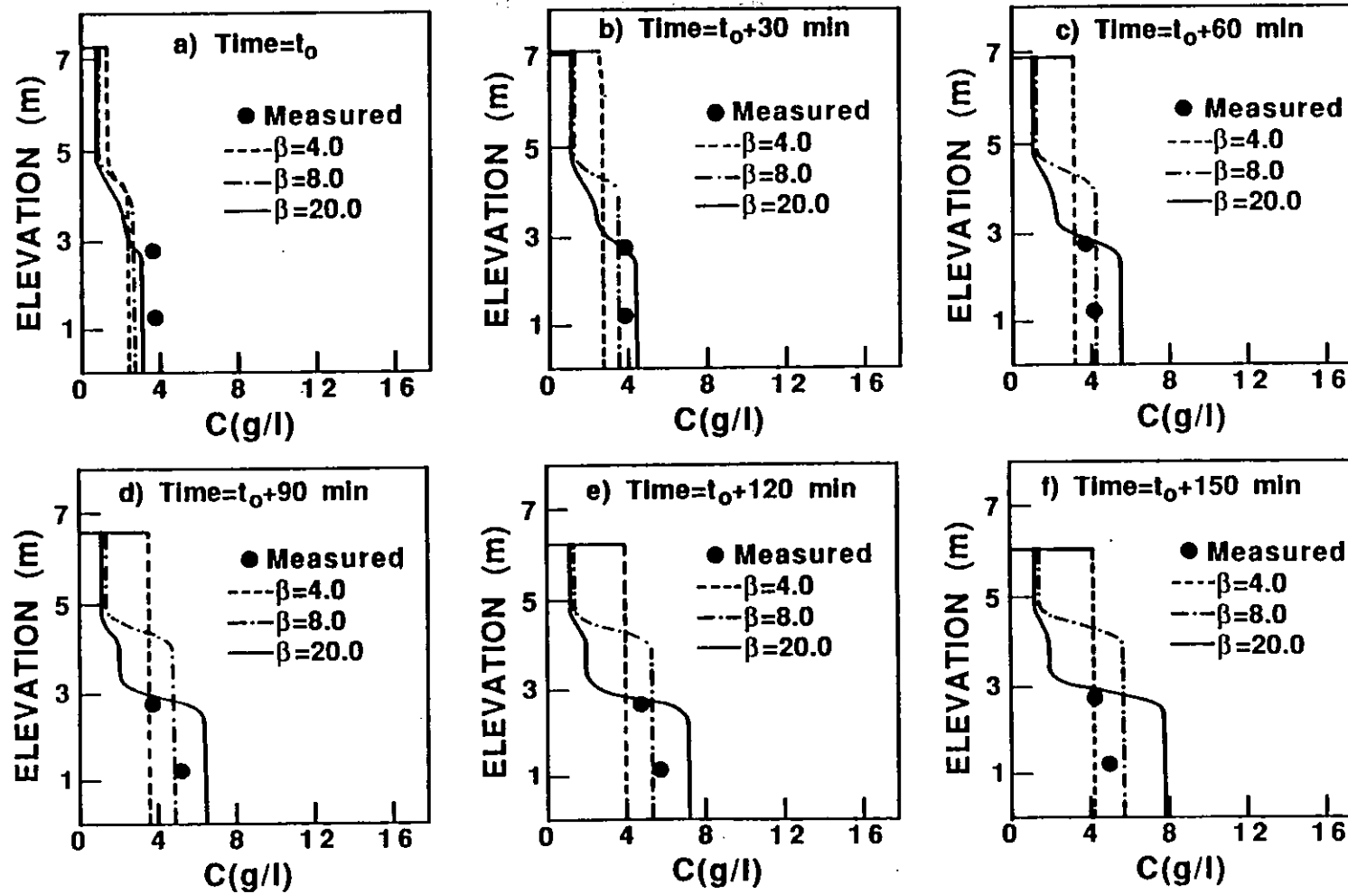
Figure 5.6: Simulated profiles with different values of \beta with high erosional fluxes at the bottom.
