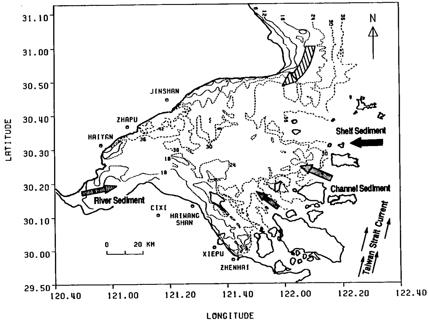
Figure 4.5: Sediment transport patterns in Hangzhou Bay. Courtesy of Dr. Hsiang Hwang.
