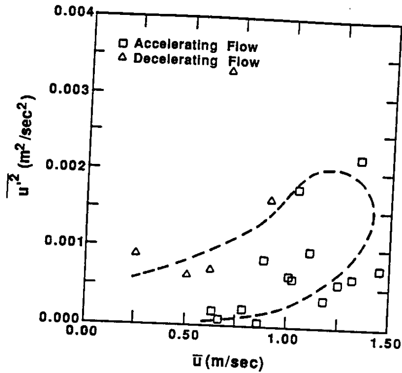
Figure 5.21: Hysteresis in u variance.
