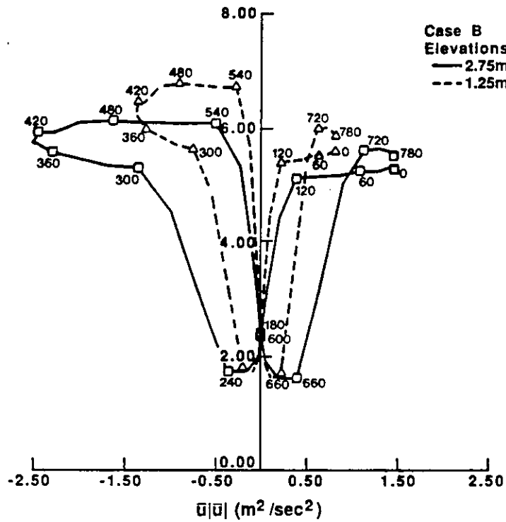
Figure 5.13: C vs. \bar{u}|\bar{u}| for case B.
