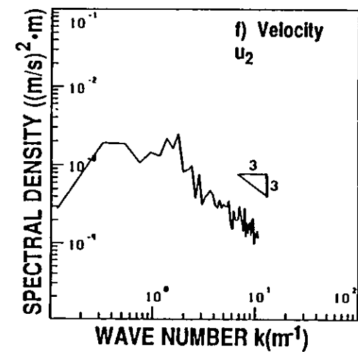
Figure 5.16: Examples of computed spectra for variables of the e_1 type. a) C_2 ; b) C_1 ; c) u_1 ; d) v_1 ; e) w_2 ; f) u_2
