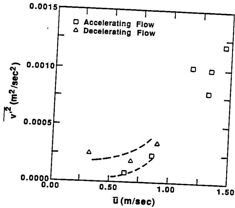
Figure 5.22: Hysteresis in v variance.
