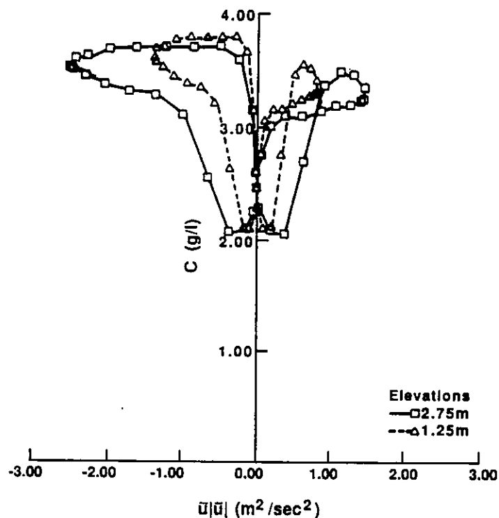
Figure 5.18: Hysteresis loops simulated using Hangzhou Bay sediment settling properties.
