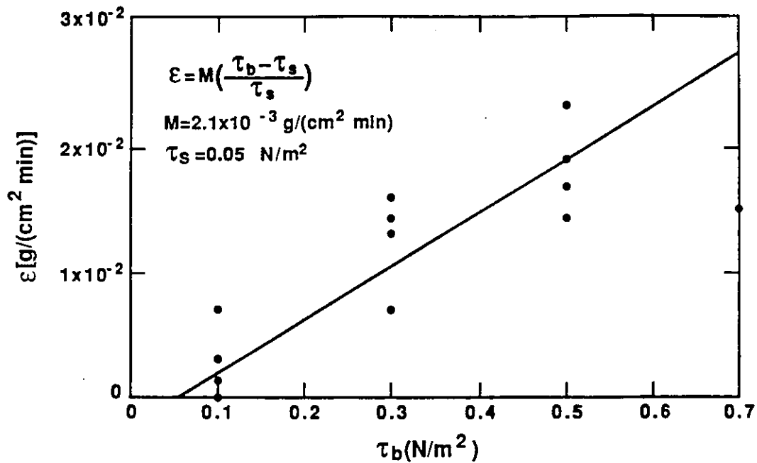
Figure 4.3: Erosion rate versus applied bottom shear stress for Hangzhou Bay sediment
