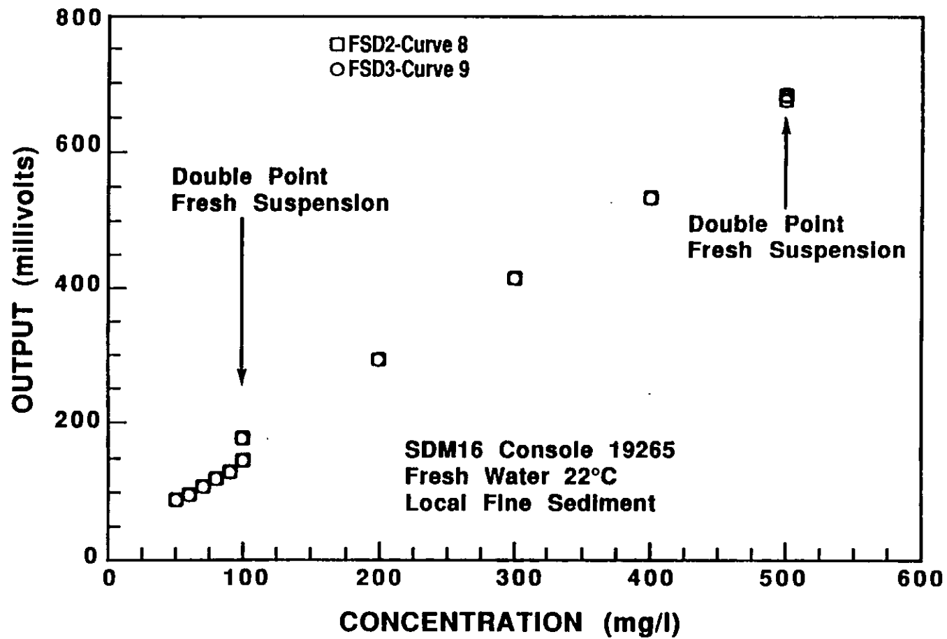
Figure A.4: Calibration curves for the SDM16 transducer and channels FSD2 and FSD3 of console 19265 using fresh water.
