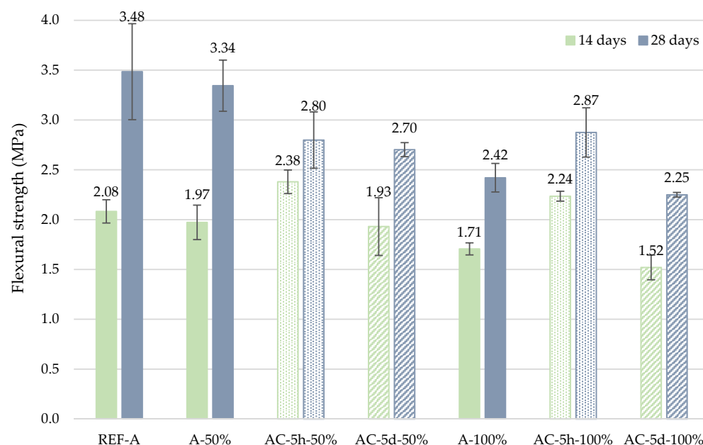
Figure 7. Flexural strength results.
