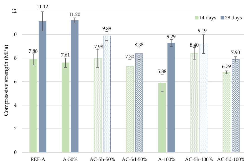
Figure 8. Compressive strength results.
