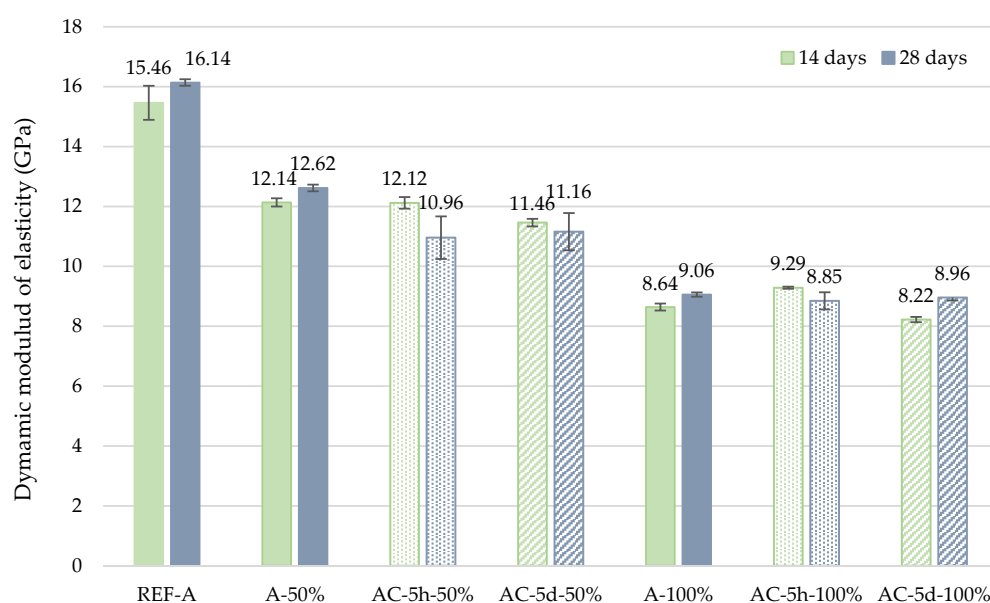
Figure 6. Dynamic modulus of elasticity results.
