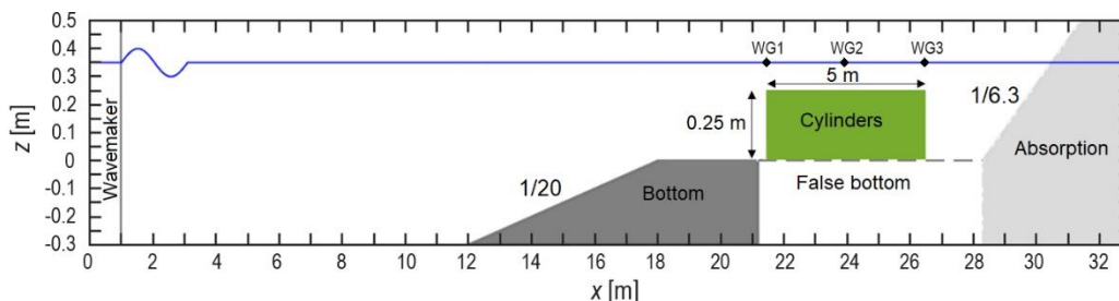
Fig. 1. Wave flume layout schematisation.
