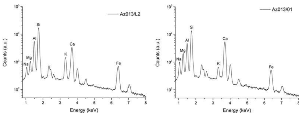
Figure 15. Relevant parts of the biscuit spectra of Az013/L2 (left) compared to Az013/01 (right) depicting the clear differences in the relative contents of Ca, Mg and K that characterize the two clusters of Figure 13
