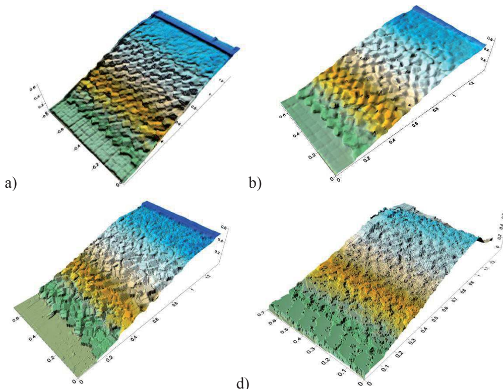
Fig. 3 Model envelope obtained with the four different methodologies. a) Kinect sensor b) MicMac software c) Python Photogrammetry Toolbox and d) Stereo photogrammetric reconstruction of submerged scenes
