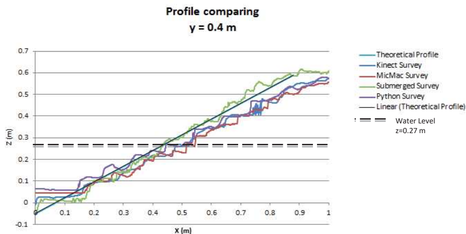
Fig. 4 Profile comparing using the four methodologies
