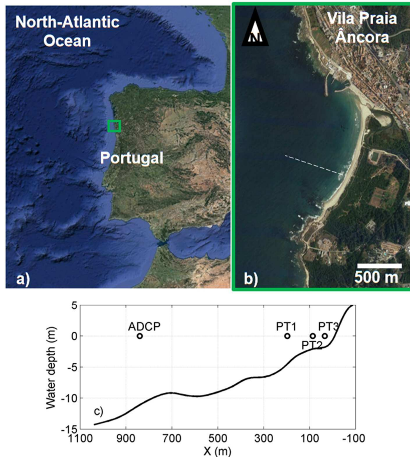
Figure 1 – Geographic location of the Vila Praia de Âncora beach (a) and b), adapted from GoogleEarth). Topobathymetric profile based on the 2011 LIDAR information and instruments positions (c)). Water depth is relative to mean sea level.
