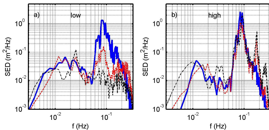
Figure 3 – Infragravity wave band spectrum for PT1 (solid blue lines), PT2 (dashed red lines) and PT3 (dashed-dot black line) during: a) low-tide, and b) high-tide.
