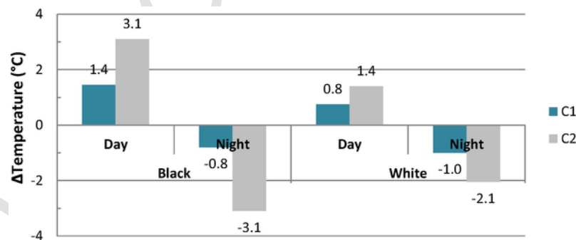
Fig. 11. Maximum and minimum thermal differentials between adherent and detached tiles on cells 1 and 2.
