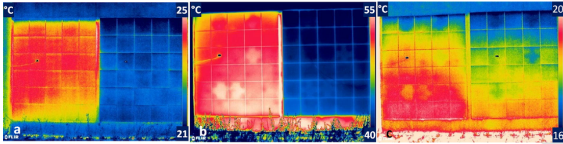
Fig. 4. C1 (ETICS) at 9:30 am (a); 3:30 pm (b) and 10:15 pm (c).
