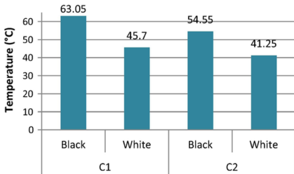
Fig. 8. Maximum average temperatures obtained in all panels' adherent tiles.
