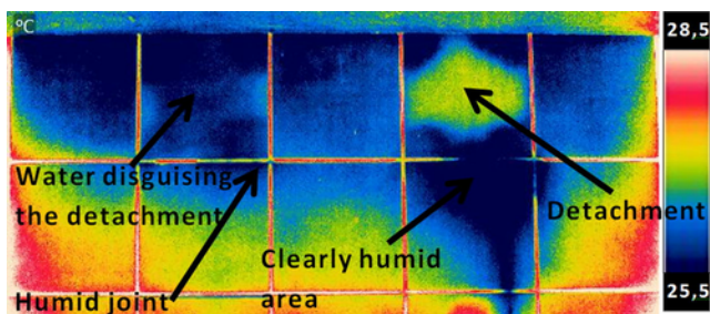
Fig. 12. Thermogram taken from C2_W at 12 pm – The classification of the anomalous tiles is presented in Table 1, where CT (second from the left) is classified with a 4 and DT (fourth from the left) with a 6.
