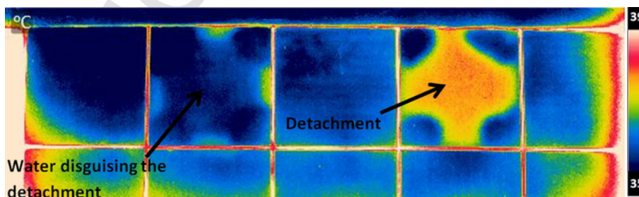
Fig. 13. Thermogram taken from C2_W at 3 pm – The classification of the anomalous tiles is presented in Table 1, where CT (second from the left) is classified with a 4&5 and DT (fourth from the left) with a 3.
