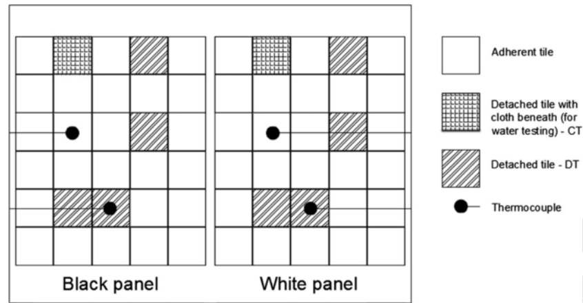
Fig. 3. Schematic representation of the panels with the detached anomalies and instrumentation.
