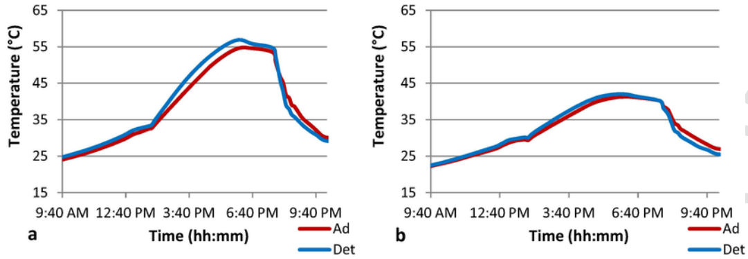
Fig. 7. Evolution of adherent (Ad) and detached (Det) tile's average temperatures in cell 2's black panel (a) and white panel (b).
