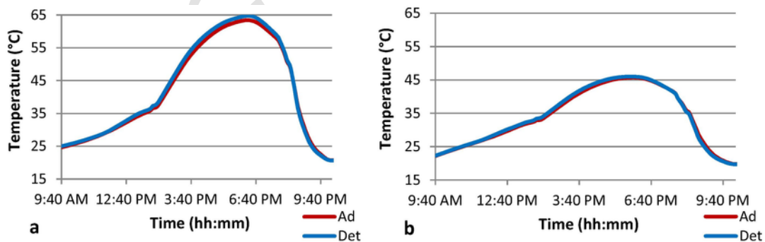
Fig. 6. Evolution of adherent (Ad) and detached (Det) tile's average temperatures in cell 1's black panel (a) and white panel (b).
