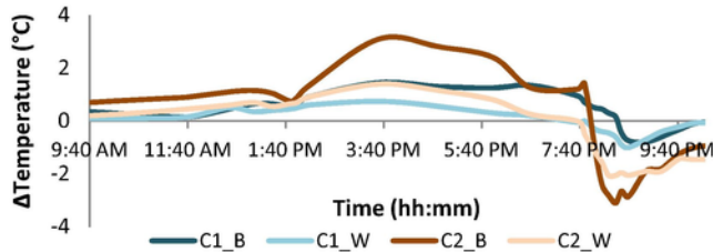
Fig. 9. Thermal differentials between detached and adherent tiles.
