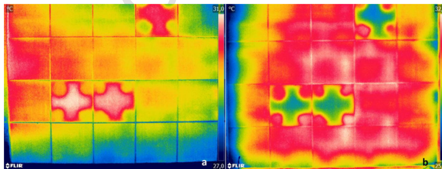
Fig. 10. Thermograms from the bottom half of cell 2's black panel taken during the day (a) and at night (b).
