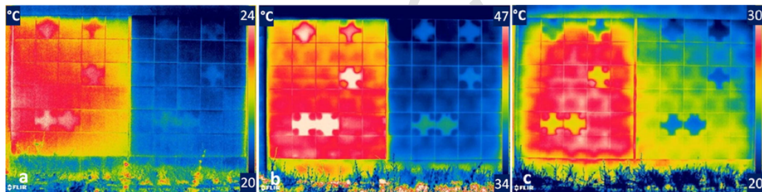
Fig. 5. C2 (rendering system) at 9:30 am (a); 3:30 pm (b) and 10:15 pm (c).
