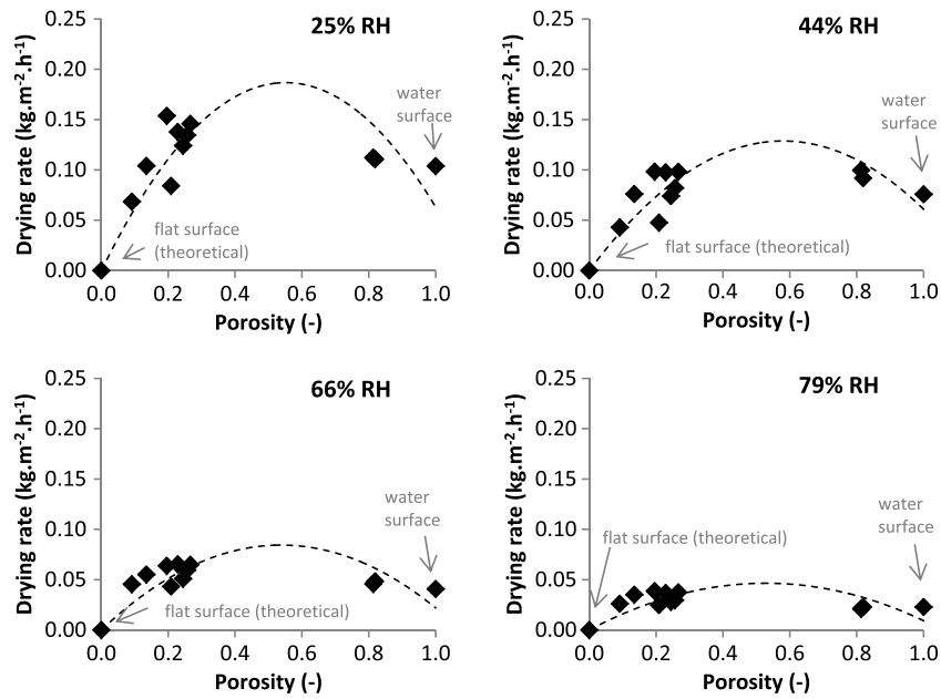
Fig. 10. Variation of the CDRP evaporation rate with the capillary porosity. The free water surface is considered a material with 100% porosity; point (0,0) is attributed to a theoretical material with 0% porosity
