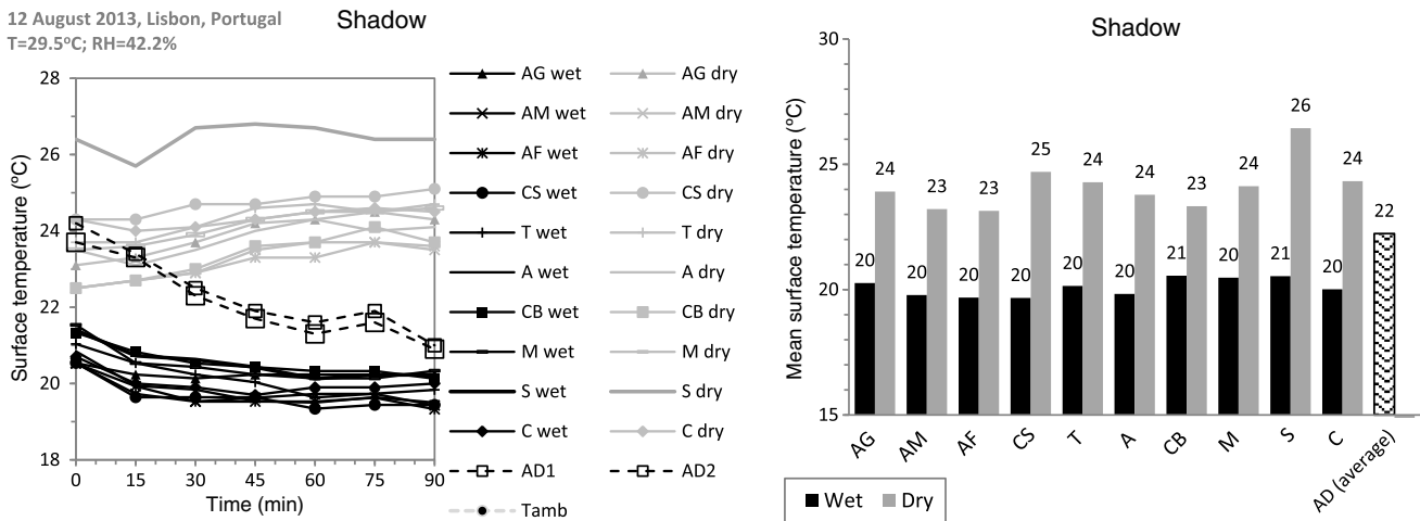
Fig. 11. Surface temperatures measured in shadow
