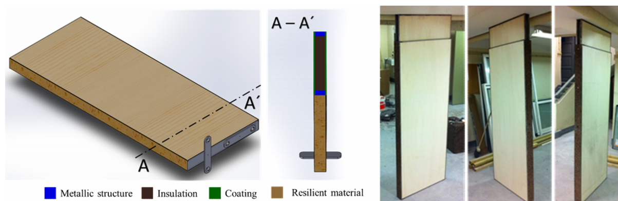
Figure 1 – Components of the module and prototype positioned in the acoustics lab of LNEC.
