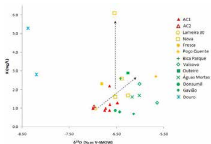
Figure 10 - Diagram K vs. \delta^{18}\text{O} for the thermal and cold groundwaters from Caldas de Moledo area.
