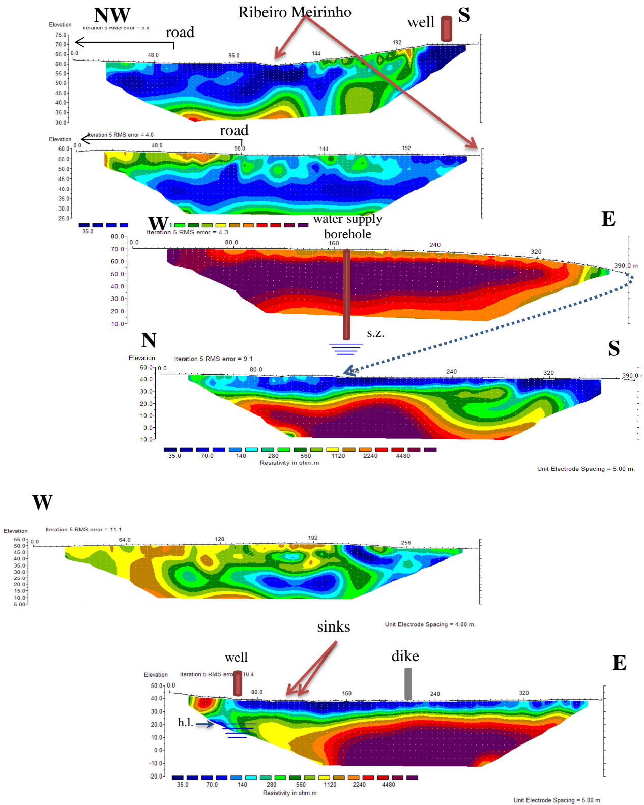
Figure 8 – Resistivity models profiles (upper-siteA: Algoz1 (top) and Algoz2 (bottom); middle-siteB: Algoz3 (top) and Algoz4 (bottom)(s.z. – top of saturated zone); bottom-siteC: Algoz5 (top) and Algoz6 (bottom))
