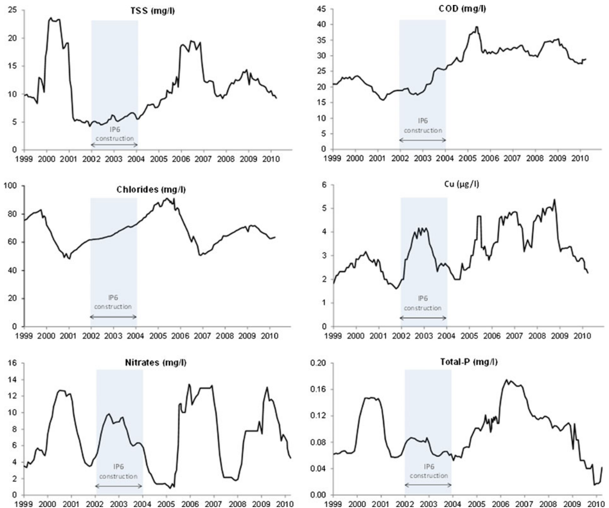
Fig. 6 Annual moving average for TSS, COD, \text{Cl}^- , Cu, \text{NO}_3^- , and Total-P concentrations in S. Domingos reservoir during the period between 1999 to 2010 (SNIRH 2010). The shaded area represents the period of construction of the IP6
