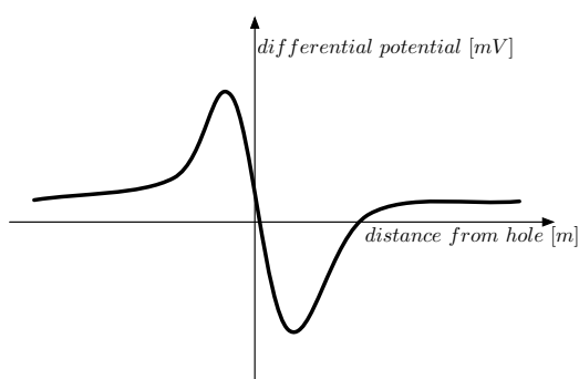
Figure 4: Electrical potential variation near a hole/defect.
