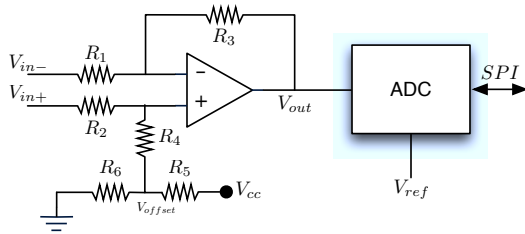
Figure 7: Signal conditioning circuit.
