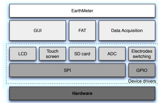
Figure 6: Software structure.
