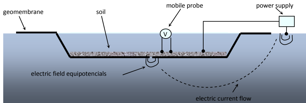
Figure 3: Mobile probe line integrity survey method.
