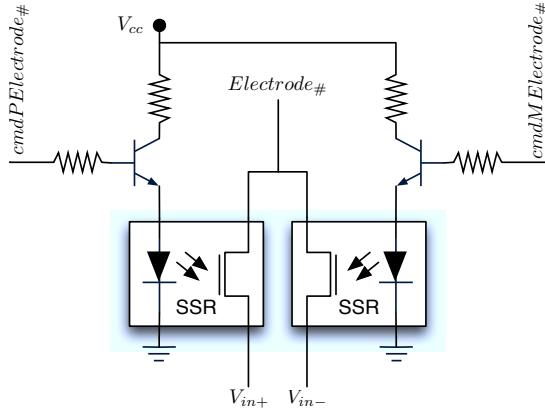
Figure 8: Switching circuit for 1 electrode.
