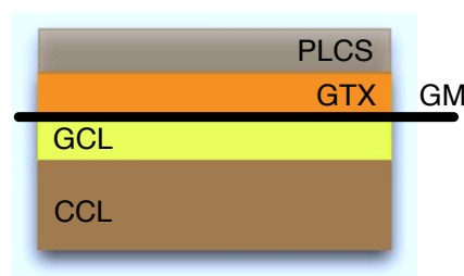
Figure 2: Landfill cut with a barrier system.
