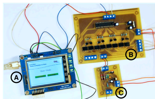
(b) Data acquisition system: A - PDI; B - Electrodes switching; C - Signal conditioning
