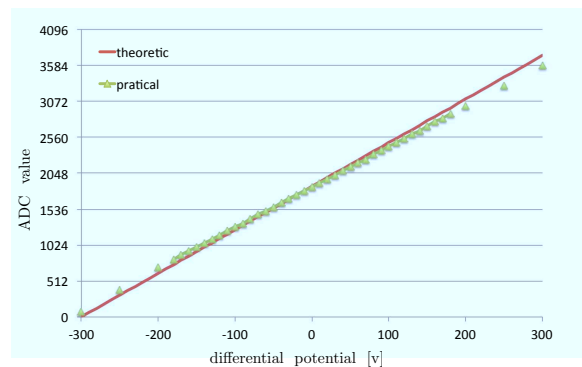
Figure 12: Characteristic of the signal conditioning module.
