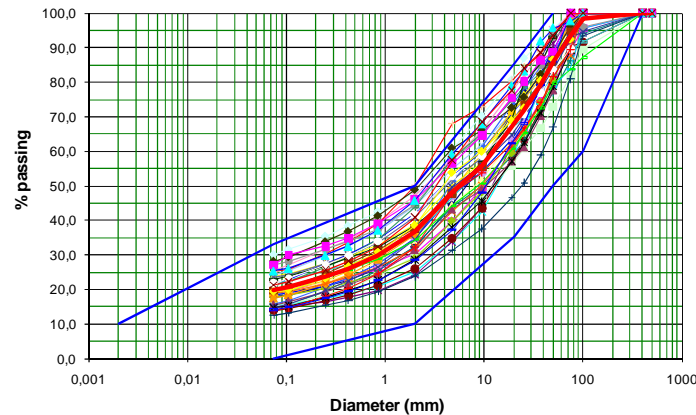
Figure 19 – Grain size distribution of shell materials of Odelouca Dam
