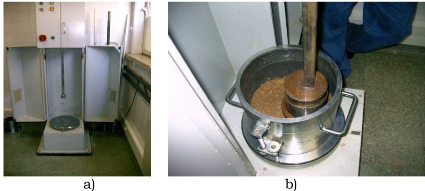
Figure 15 – a) Toni-tecnik compactor, b) mould and the pestle use in the standard compaction tests.
