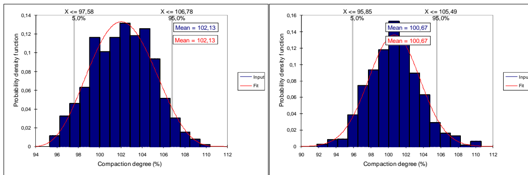
Figure 21 – Histogram and density probability functions of the compaction degree of Odelouca dam: a) upstream shell; b) downstream shell.
