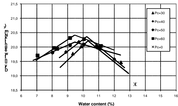
Figure 16 – Compaction curves from standard compaction tests
