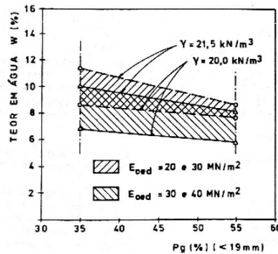
Figure 8 – Correlations between water content, dry density, percent of coarser fraction and oedometric modulus for Meimoa dam (JAE/LNEC, 1994)
