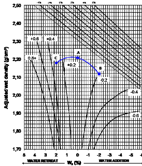
Figure 20 – Hilf's method graphic
