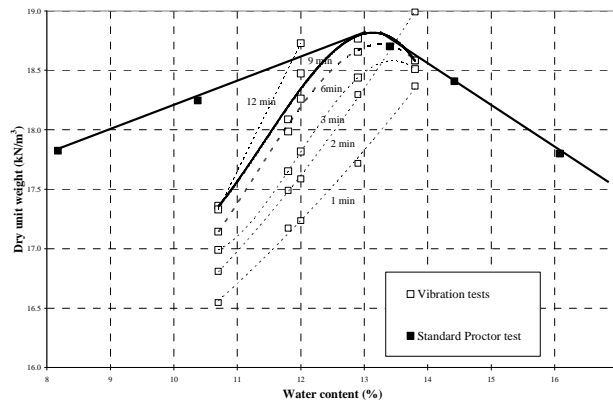
Figure 13 – Comparison of the compaction curves obtained by vibration and by the standard Proctor test (Caldeira and Brito, 2007)
