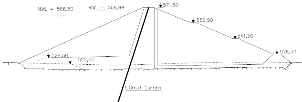
Figure 5 – Cross-section of Meimoa dam
