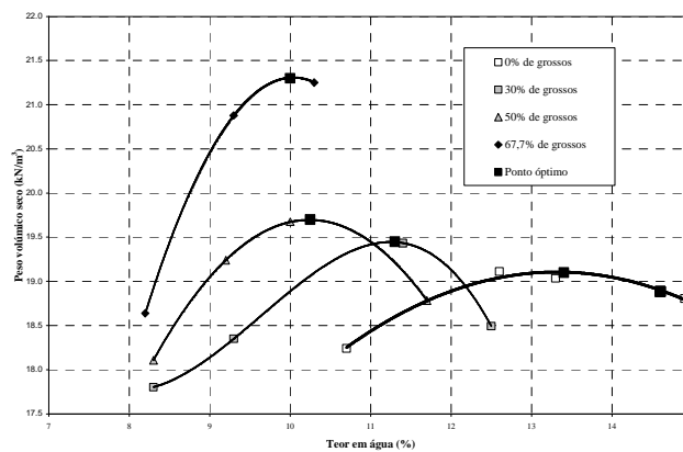
Figure 14 – Joint representation of compaction curves, after nine minutes of vibration, and their optimum points
