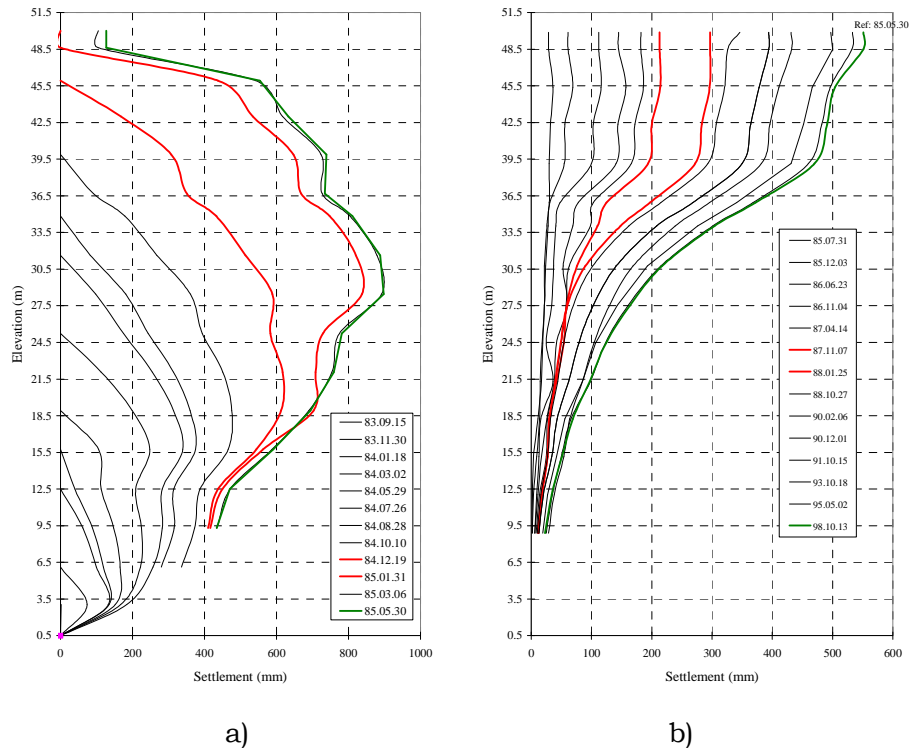
Figure 4 – Vertical displacements at A1 settlement gauge during: a) construction; b) first filling of the reservoir
