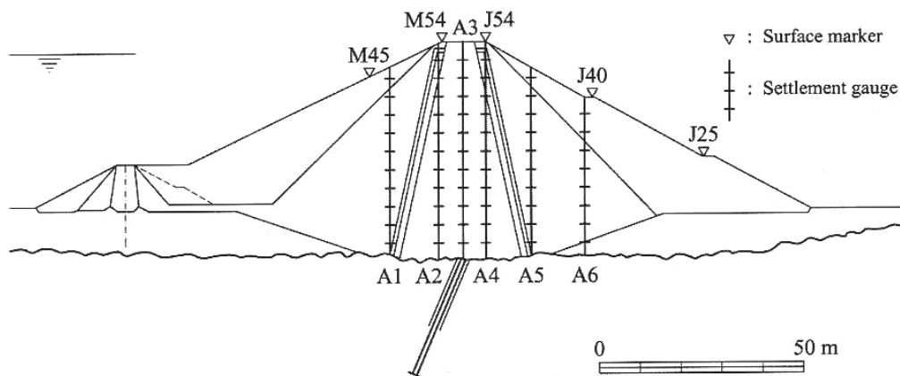
Figure 3 – Settlements gauges at cross-section 7
