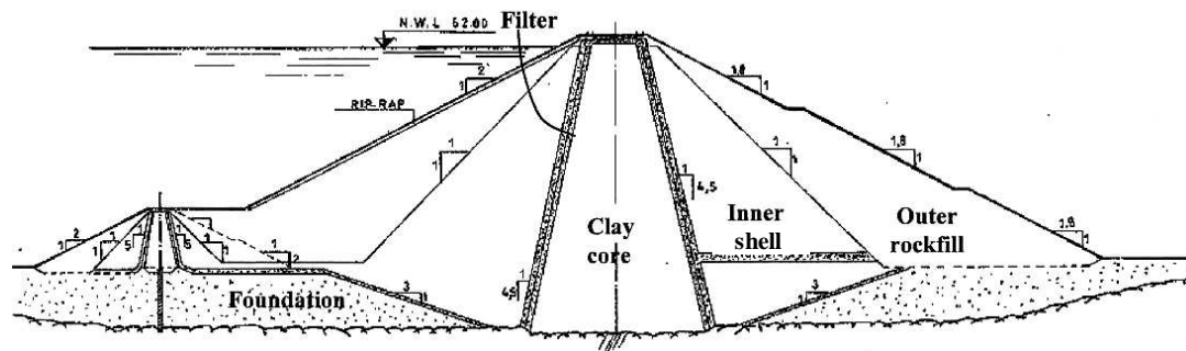
Figure 2 – Cross-section of Beliche dam
