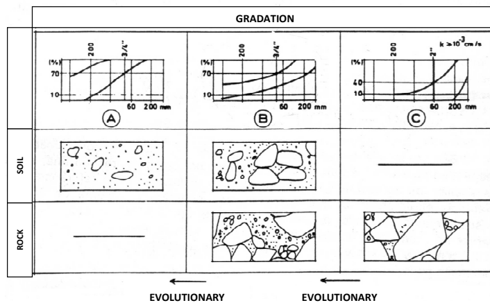
Figure 1 – Typical grain size distribution and structure of (Maranha das Neves, 1993) of: A) soils; B) soil-rock mixtures; C) rock fill.
