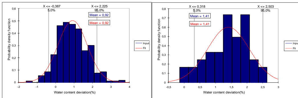
Figure 22 – Histogram and density probability functions of the water content deviation of Odelouca Dam: a) upstream shell; b) downstream shell
