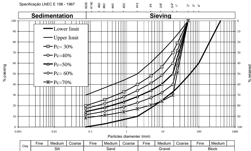
Figure 12 – Grain size distributions of mixtures with particles limited to 2” with varying percentages of the coarse fraction
