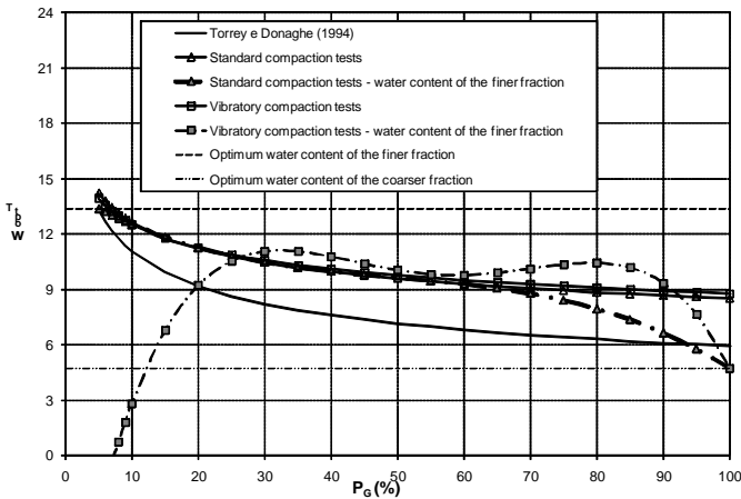
Figure 18 – Optimum water content of total material as function of the coarser fractions
