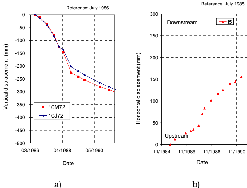
Figure 7 – Displacements during first filling a) settlements of crest markers; b) top horizontal displacement of an inclinometer
