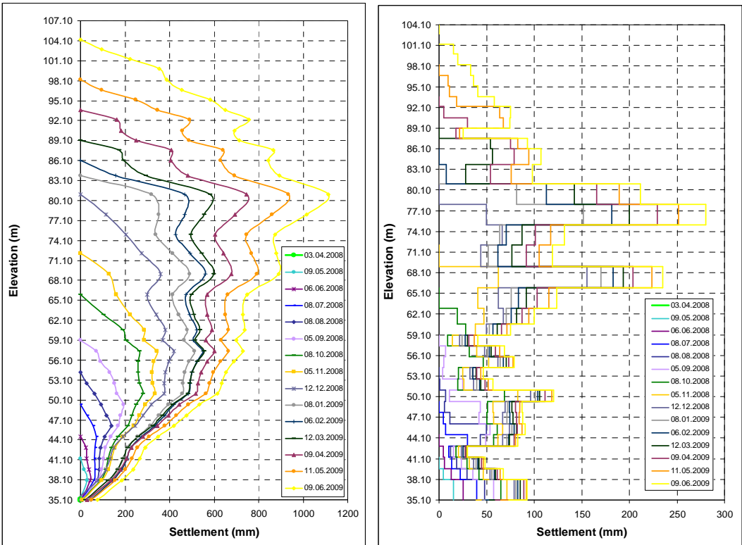
Figure 23 – Settlements during Odelouca dam construction: a) accumulated; b) incremental
