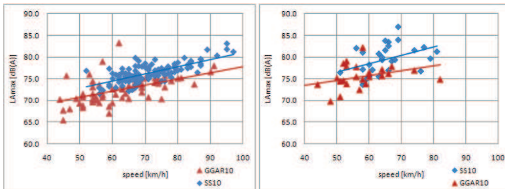
Figure 1 - Example of data results for light (left) and L2a type heavy vehicles (right)
