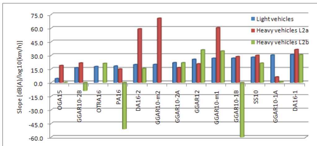
Figure 2 - Slope of the curve L_{max} versus log 10 of speed for heavy and light vehicles
