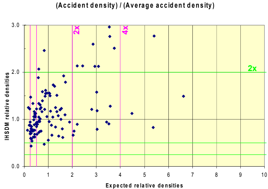
FIGURE 4 Comparison of accident densities on horizontal curves.
